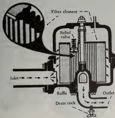
FIGURE 3-56. Aircraft fuel filter.
